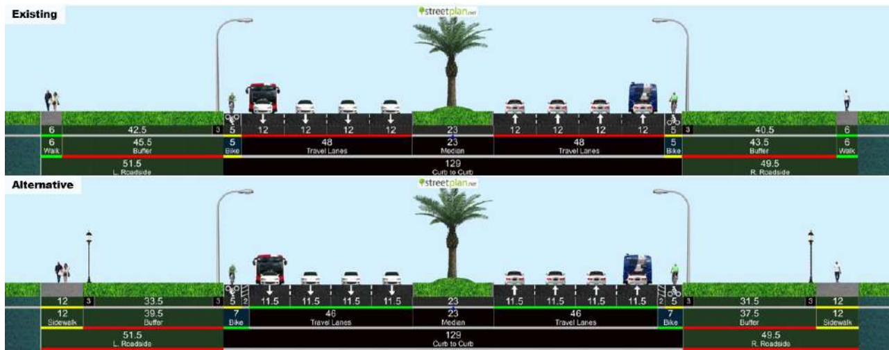
Figure 3. MCS Mixed Traffic Bus Alternative Concept
