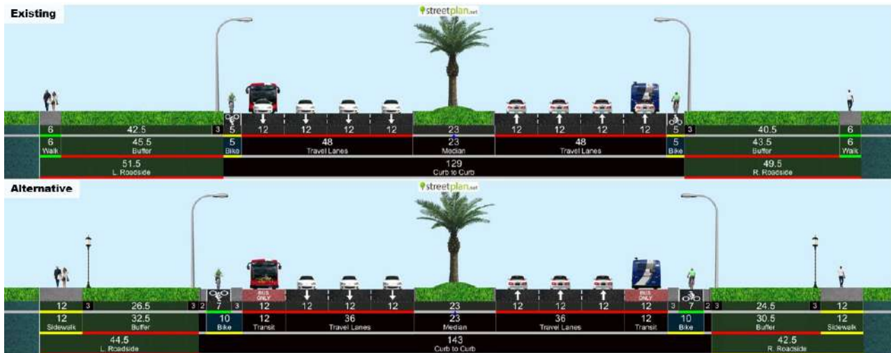
Figure 5. Dedicated BRT Lane Alternative Concept
