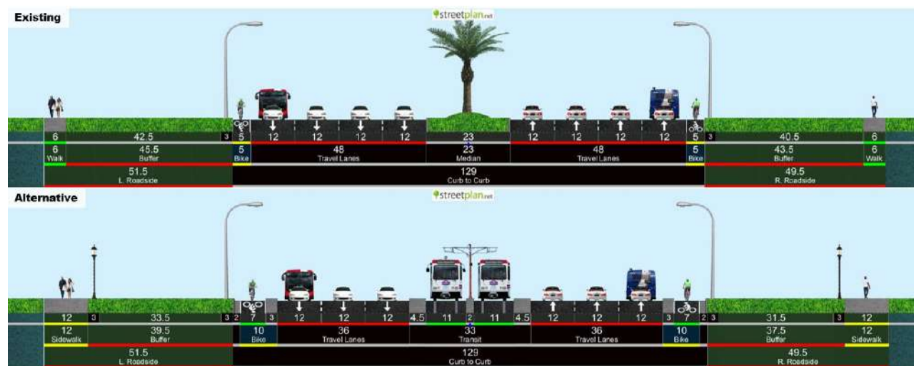
Figure 7. Dedicated Lane LRT Alternative Concept
