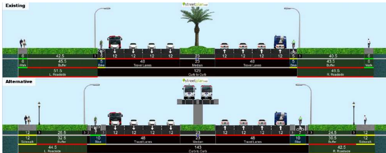
Figure 8. Elevated LRT Alternative Concept
