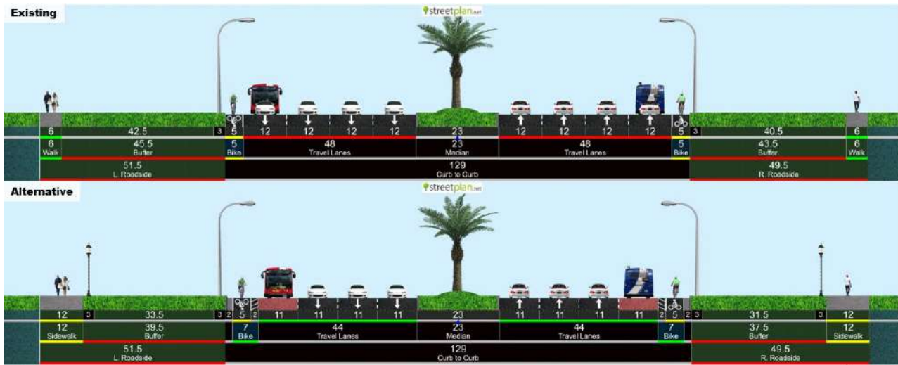
Figure 4. MCS BAT Lane Alternative Concept
