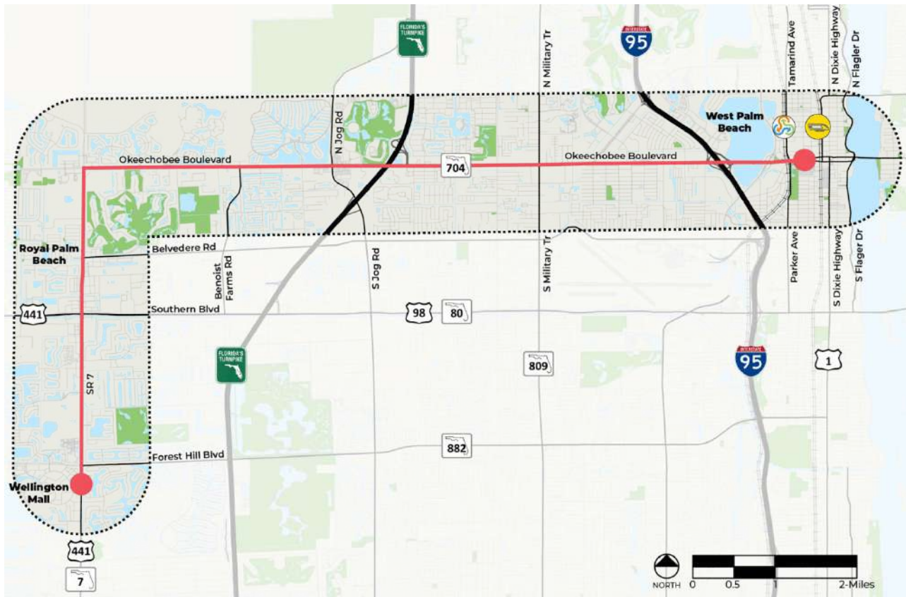
Figure 1. Okeechobee Blvd. & SR 7 MCS
