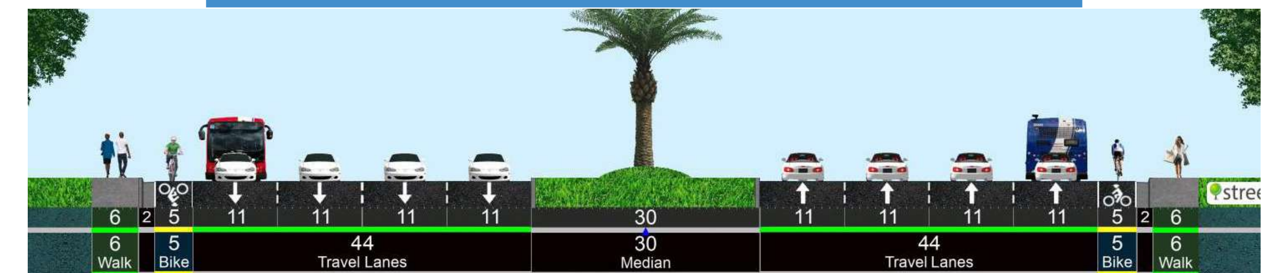
Australian Ave to Tamarind Ave Right-of-Way: 144 feet
