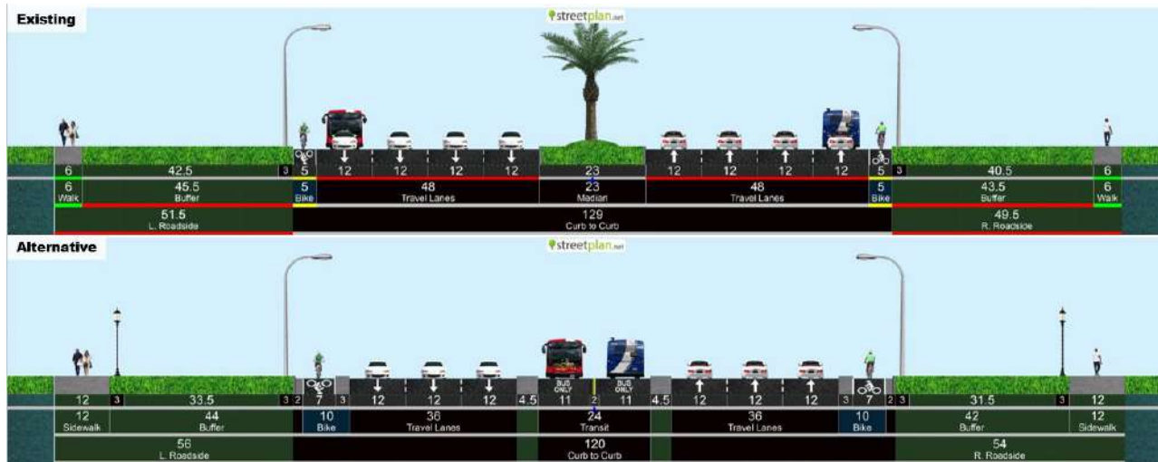
Figure 6. MCS Center Platform Dedicated Lane BRT Alternative Concept
